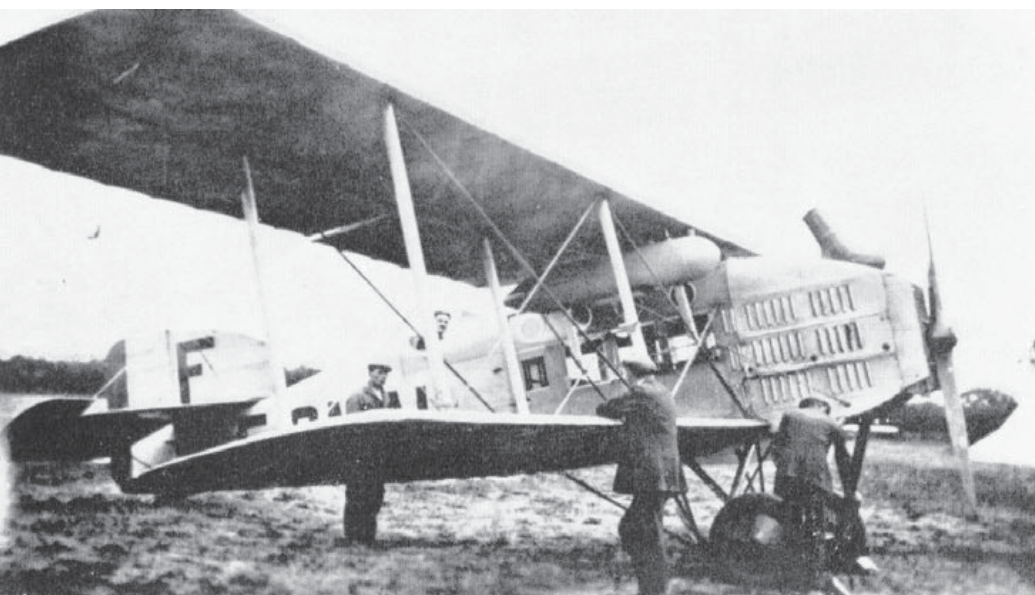
Breguet 14Tbis with the improved cabin arrangements and additional windows that distinguished it from the 14T. The bracing of the interplane fuel tanks to the intersections of the flying and landing wires is noteworthy.
