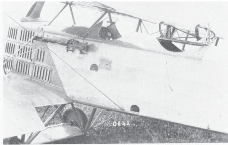
Close-up of cockpits on early Breguet 14A2, probably No. 665. The gun mounting on the rear cockpit is a T.O.4. (Photo: Musée de l'Air 0842)
