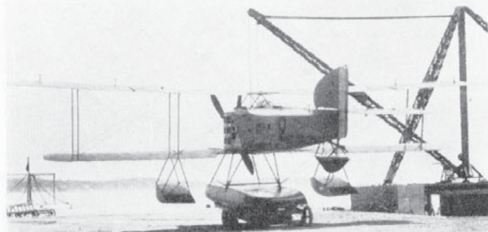
Breguet 14H. The aircraft has horn-balanced ailerons and wire trailing edges on the mainplanes; the lower wing appears to be that of a 14A2, yet the fuselage has the side windows of a 14B2.
