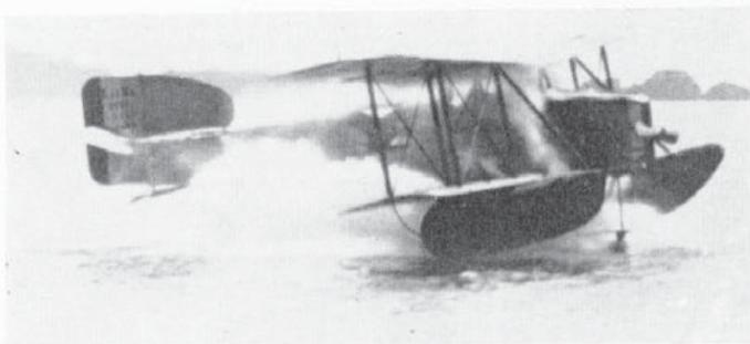
Breguet 14B2 fitted with flotation gear. The aircraft has horn-balanced ailerons, wire trailing edges, the late 14B2 lower wing and underwing skids.
